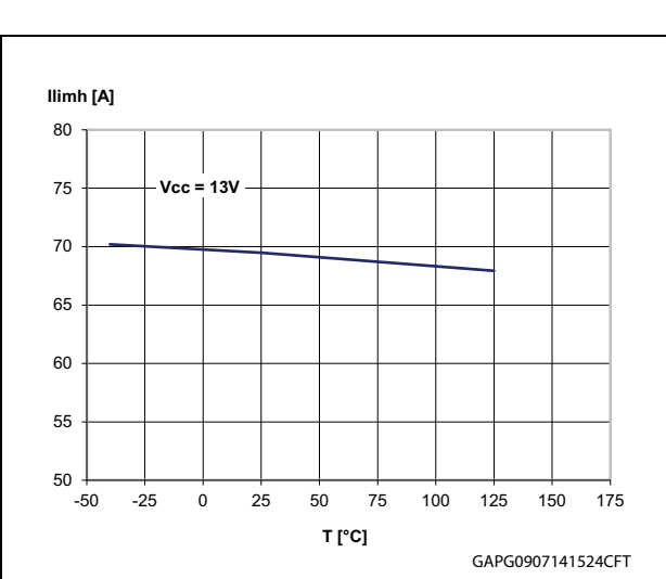
Figure 26. I_{LIMH} vs. T_{case}
