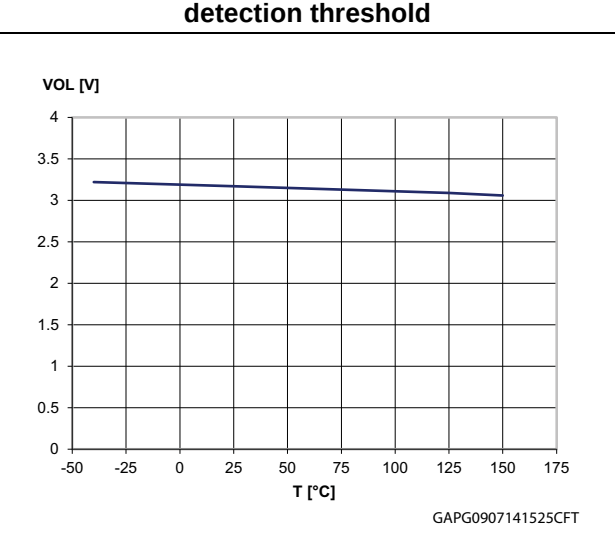
Figure 27. OFF-state open-load voltage detection threshold
